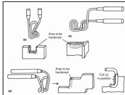
Fig. 6: Coil modifications for localized heating (from F. W. Curtis, High Frequency Induction Heating , McGraw-Hill, New York, 1950)
