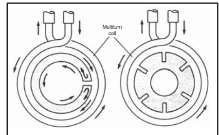
Fig. 16: Localized overheating of slots in certain parts that results from the tendency for induced currents to follow the part contour (from F. W. Curtis, High Frequency Induction Heating , McGraw-Hill, New York, 1950)
