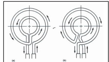
Fig. 18: Design of pancake coils to provide (a) uniform, or overall, heating or (b) peripheral heating only (from F. W. Curtis, High Frequency Induction Heating , McGraw-Hill, New York, 1950)
