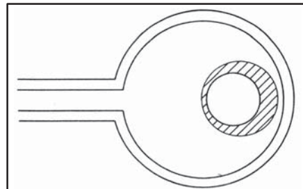
Fig. 2: Induction heating pattern produced in a round bar placed off center in a round induction coil.
