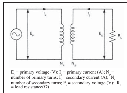
Fig. 1: Electrical circuit illustrating the analogy between induction heating and the transformer principle.
