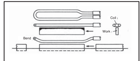
Fig. 9: Typical channel coil used to heat the edges of discrete lengths of rectangular bar stock; end of coil is decoupled by bending to prevent overheating of ends (from F. W. Curtis, High Frequency Induction Heating , McGraw-Hill, New York, 1950)
