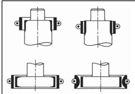
Fig. 13: Effect of coil placement on the heating pattern at the end of a workpiece (from F. W. Curtis, High Frequency Induction Heating , McGraw-Hill, New York, 1950)
