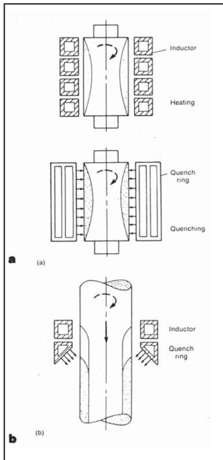
Fig. 3: Inductor/quench designs for induction scanning: (a) separate coil and quench; and (b) two-chamber, integral coil and quench (from F.H. Reinke and W. H. Gowan, Heat Treatment of Metals , Vol. 5, No. 2, 1978, p. 39)
