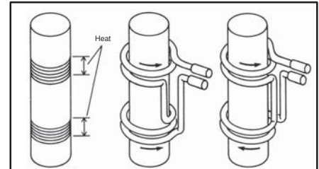
Fig. 17: Control of heating patterns in two different regions of a workpiece by winding the turns in opposite directions (from F. W. Curtis, High Frequency Induction Heating , McGraw-Hill, New York, 1950)
