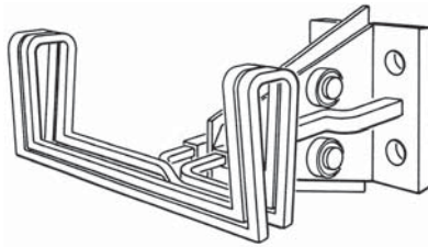
Fig. 11: Multiturn channel coil used to increase the ampere turns coupled to an induction heated workpiece (source: Lindberg Cycle-Dyne Inc.)
